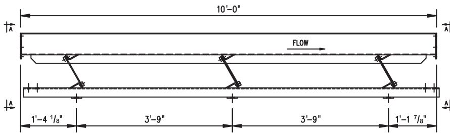
STANDARD EXTENSION SECTION
