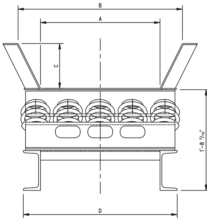
COILWEB® UNBALANCED
