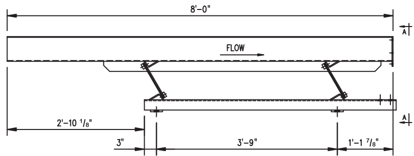
FEED END EXTENSION SECTIONS
